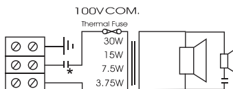
MSH30T/ENC *with capacitor
